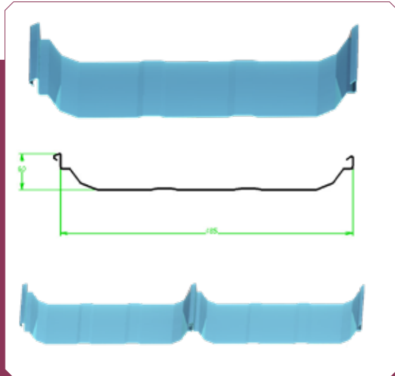
SEAMLOCK TOLE
