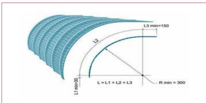
STEEL ARCH ROOF
