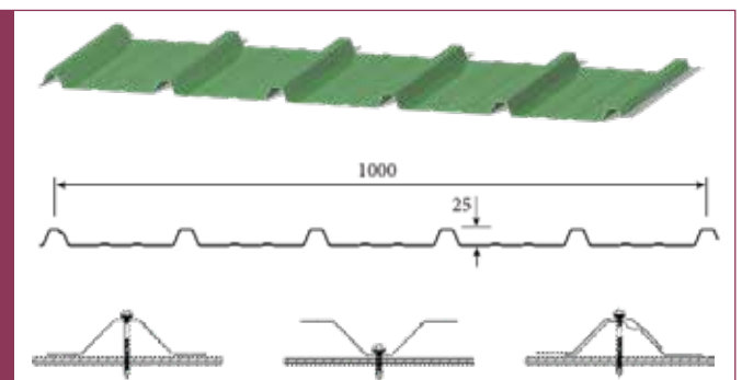
SIX-CORRUGATION TOLE
