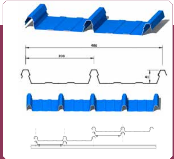
CLIPLOCK TOLE
